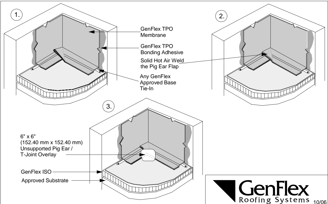
One-Piece Inside Corner with Pig Ear Overlay
