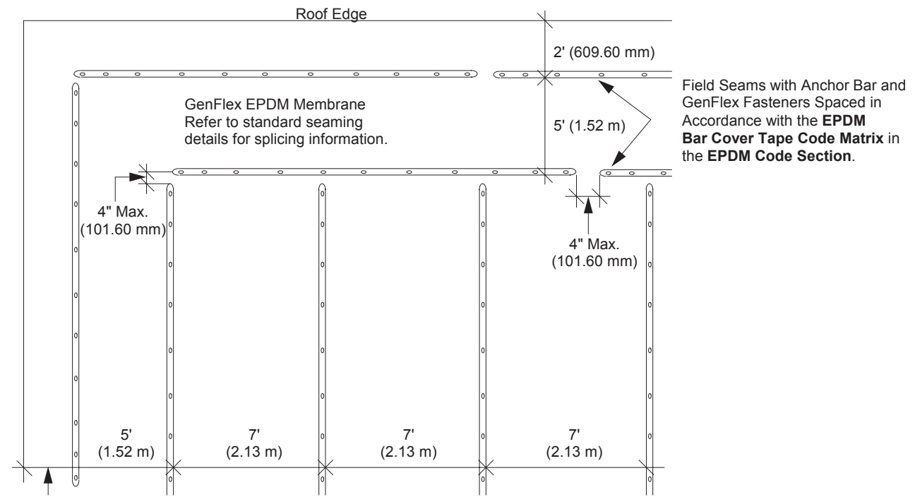
7' 0" (2.13 m) Bar Cover Tape System Perimeter Layout Pattern
