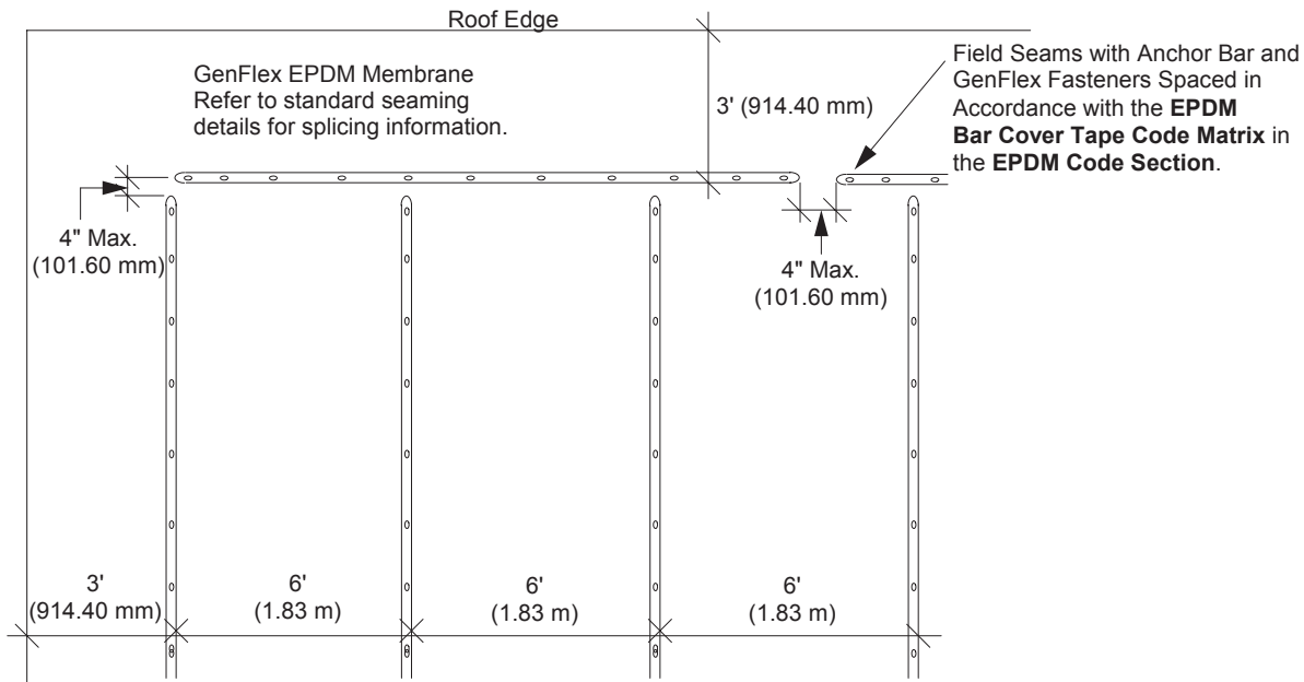
6' 0" (1.83 m) Bar Cover Tape System Perimeter Layout Pattern
