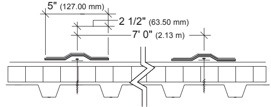
7' 0" (2.13 m) Bar Cover Tape System Layout Pattern
