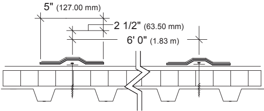
6' 0" (1.83 m) Bar Cover Tape System Layout Pattern
