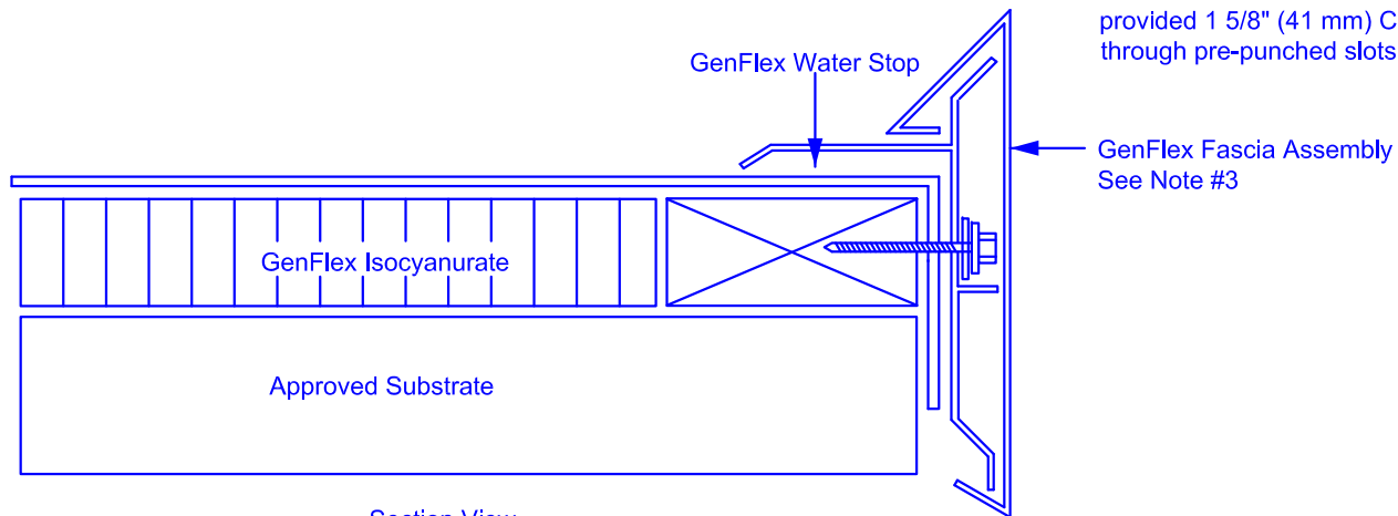
Section View
