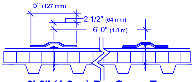
6' 0" (1.8 m) Bar Cover Tape System Layout Pattern
