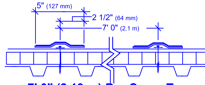
7' 0" (2.13 m) Bar Cover Tape System Layout Pattern
