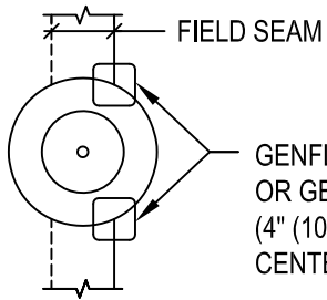
PLAN VIEW PIPE FLASHING OVER SEAM
