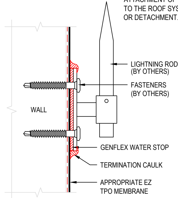
WALL MOUNT
