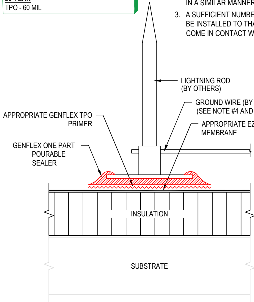
ROOF MOUNT
