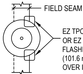
PLAN VIEW PIPE FLASHING OVER FIELD SEAM
