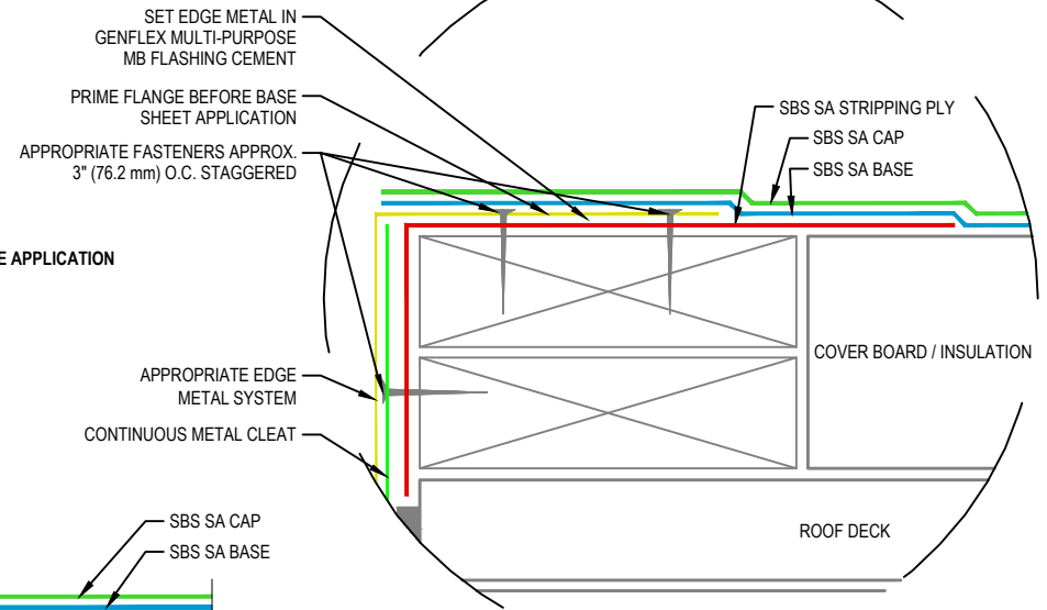
DETAIL A-1 ROOF EDGE METAL FLASHING ALTERNATIVE
